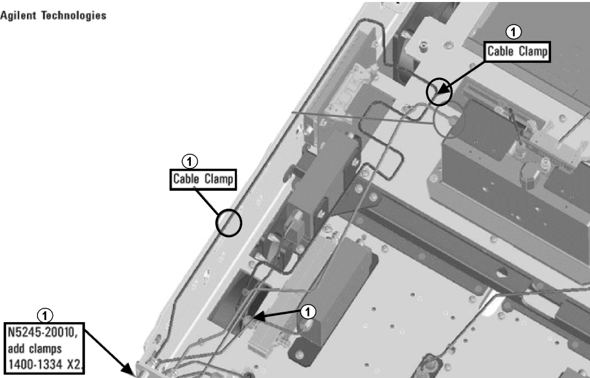
Figure 3 Location of Cable Clamps to Secure W33 (N5245-20010)
